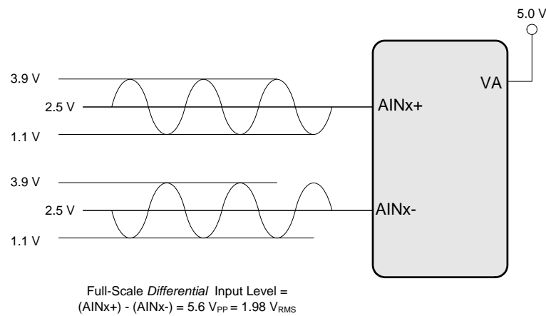
Figure 10. Full-Scale Input
