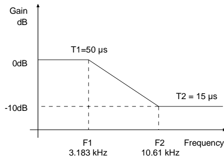
Figure 14. De-Emphasis Curve
